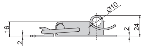
CKC-1047-2
